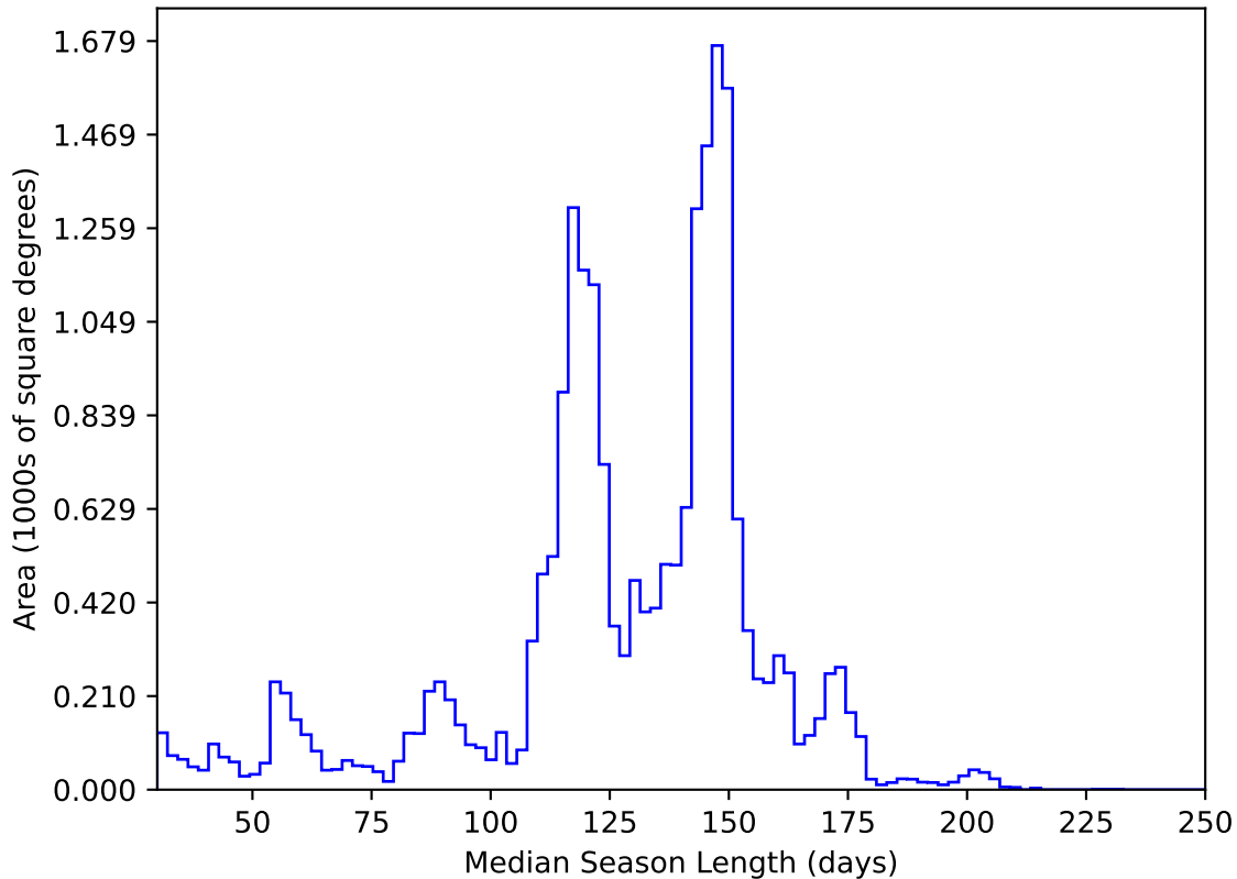
too_elab_heavy_r32_d3_ugrizy_v3.4_10yrs All sky y band: Median Season Length
