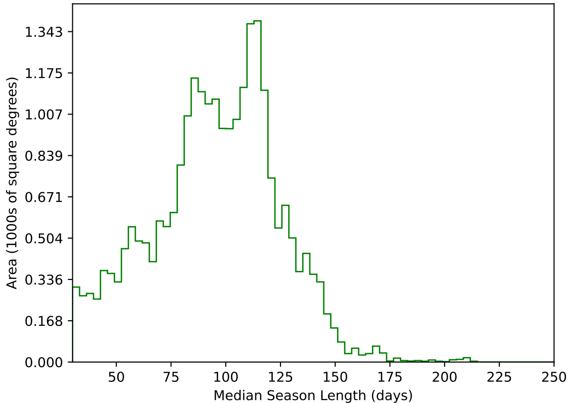
too_elab_heavy_r32_d3_ugrizy_v3.4_10yrs All sky g band: Median Season Length
