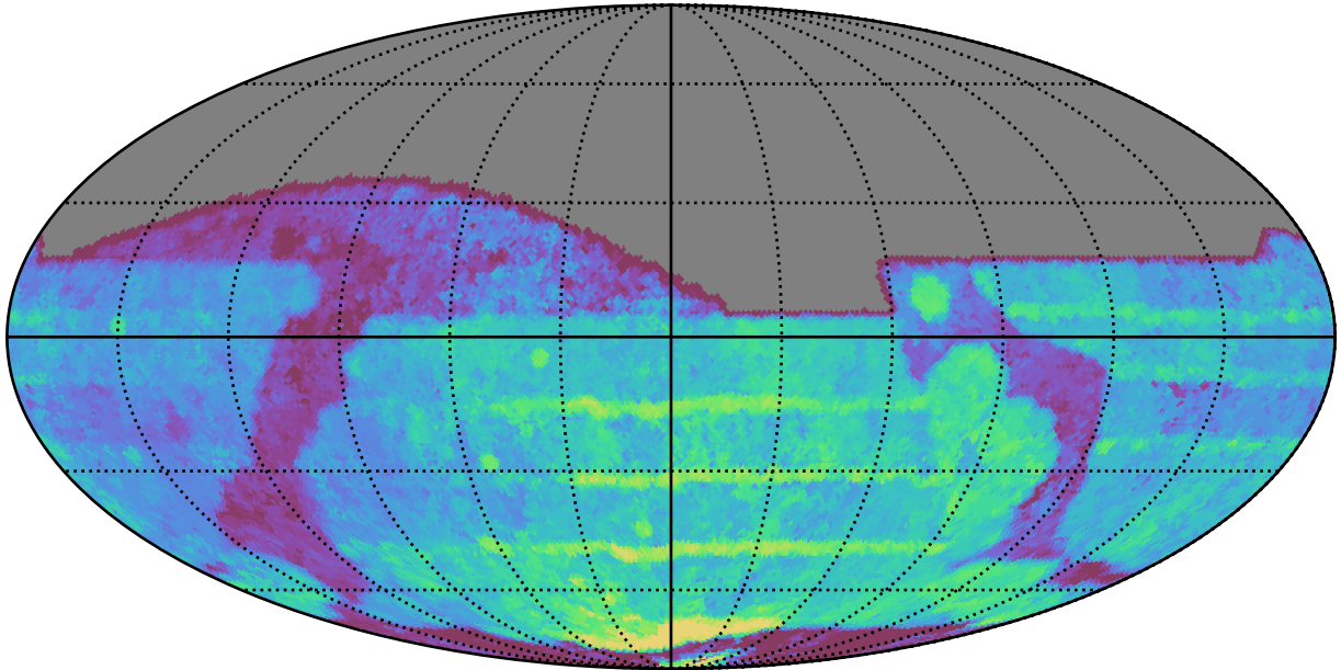
too_elab_heavy_r32_d3_ugrizy_v3.4_10yrs All sky all bands: Median Season Length
