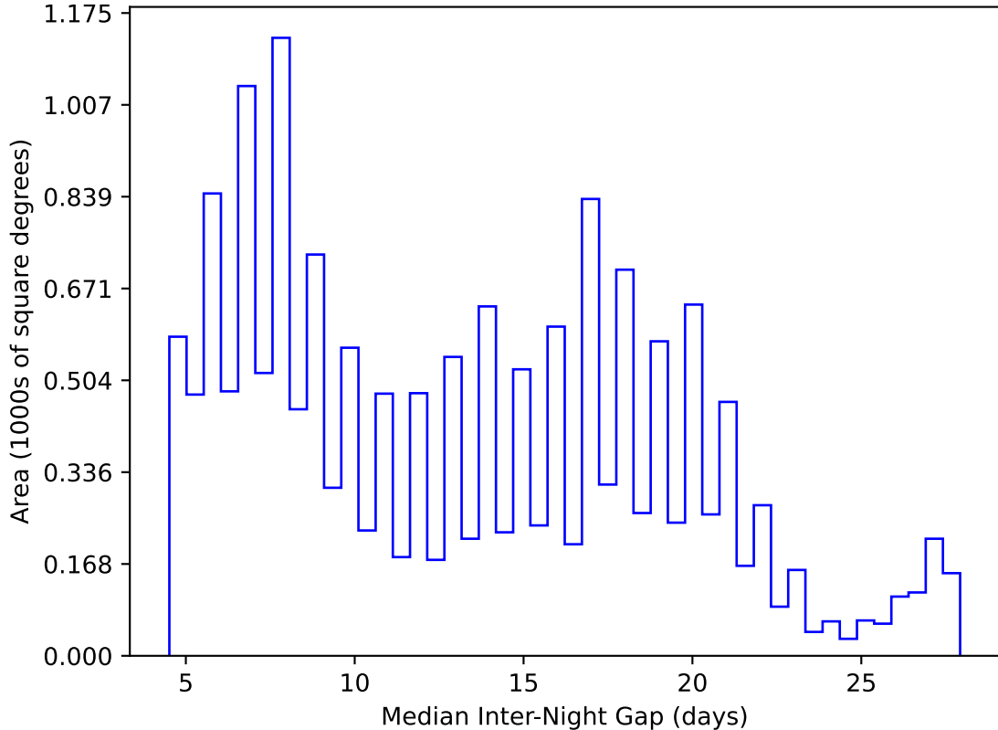
too_elab_heavy_r32_d3_ugrizy_v3.4_10yrs WFD y band: Median Inter-Night Gap
