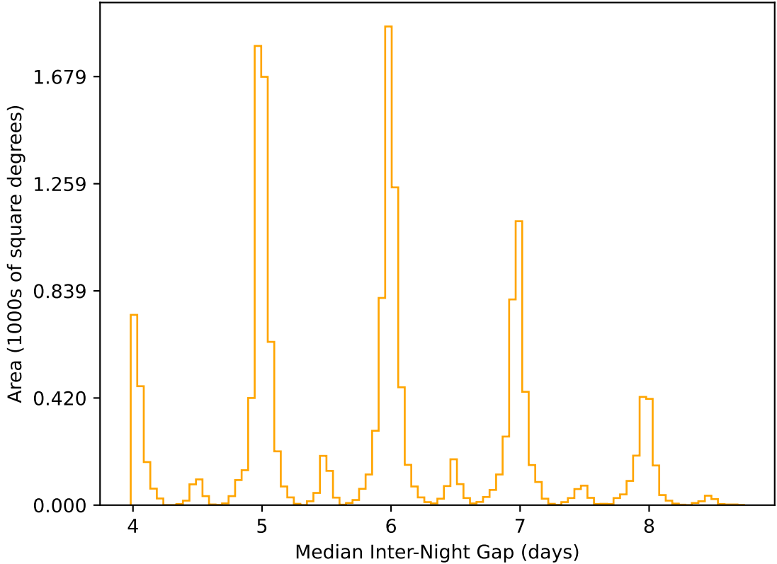
too_elab_heavy_r32_d3_ugrizy_v3.4_10yrs WFD r band: Median Inter-Night Gap
