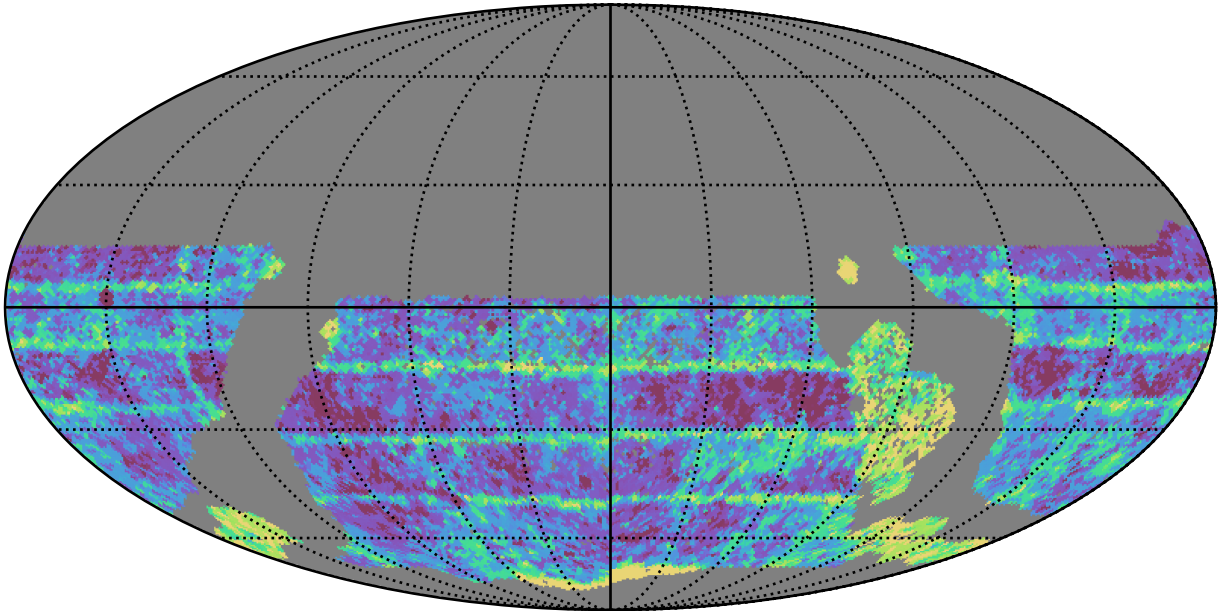
too_elab_heavy_r32_d3_ugrizy_v3.4_10yrs WFD i band: Median Inter-Night Gap
