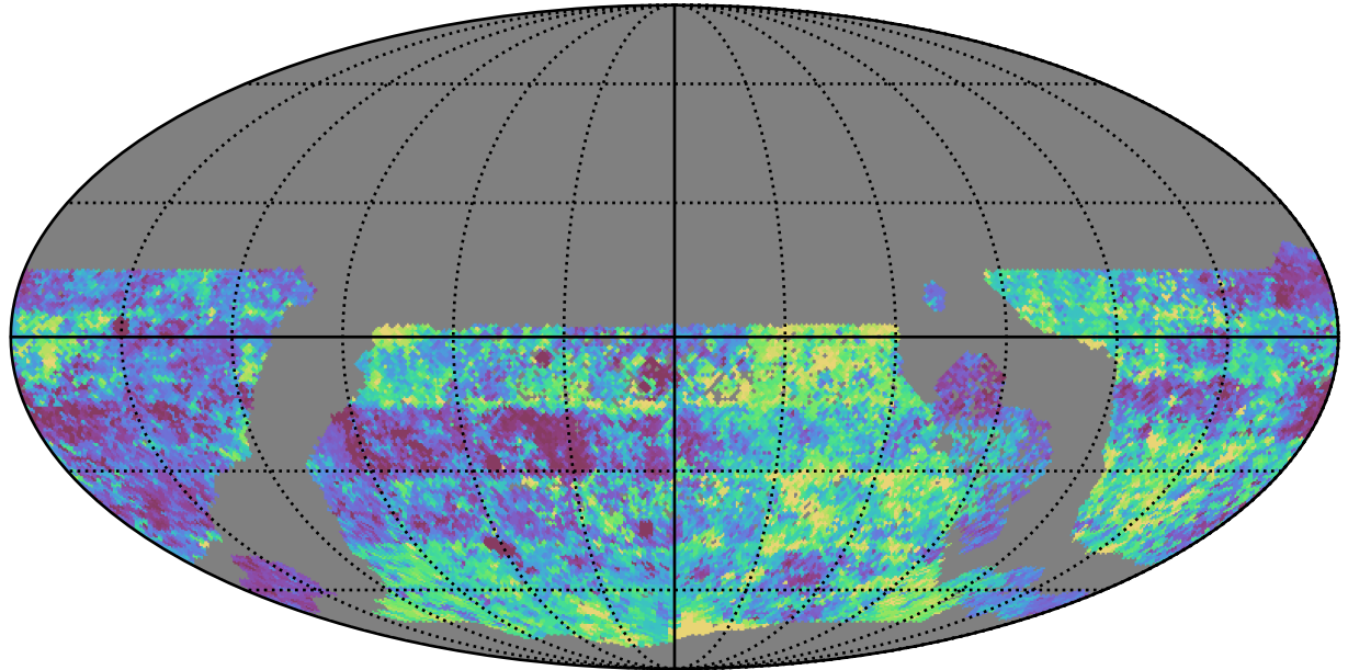
too_elab_heavy_r32_d3_ugrizy_v3.4_10yrs WFD g band: Median Inter-Night Gap
