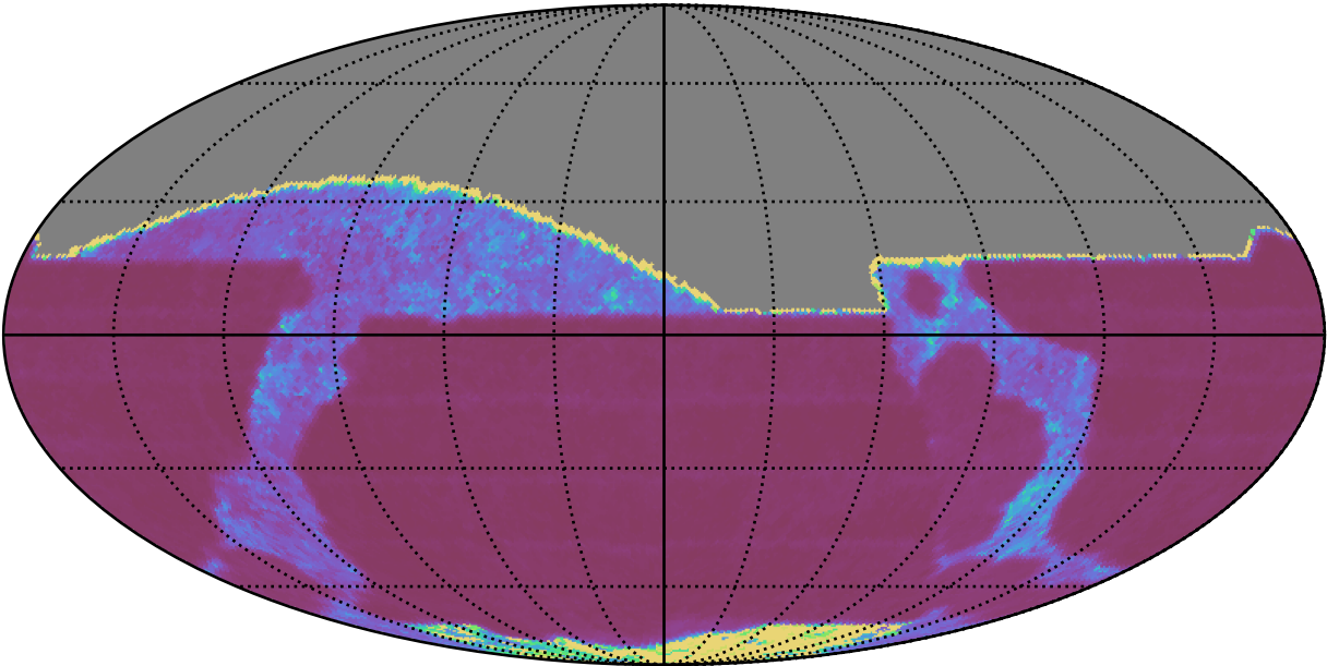
too_elab_heavy_r32_d3_ugrizy_v3.4_10yrs All sky i band: Median Inter-Night Gap
