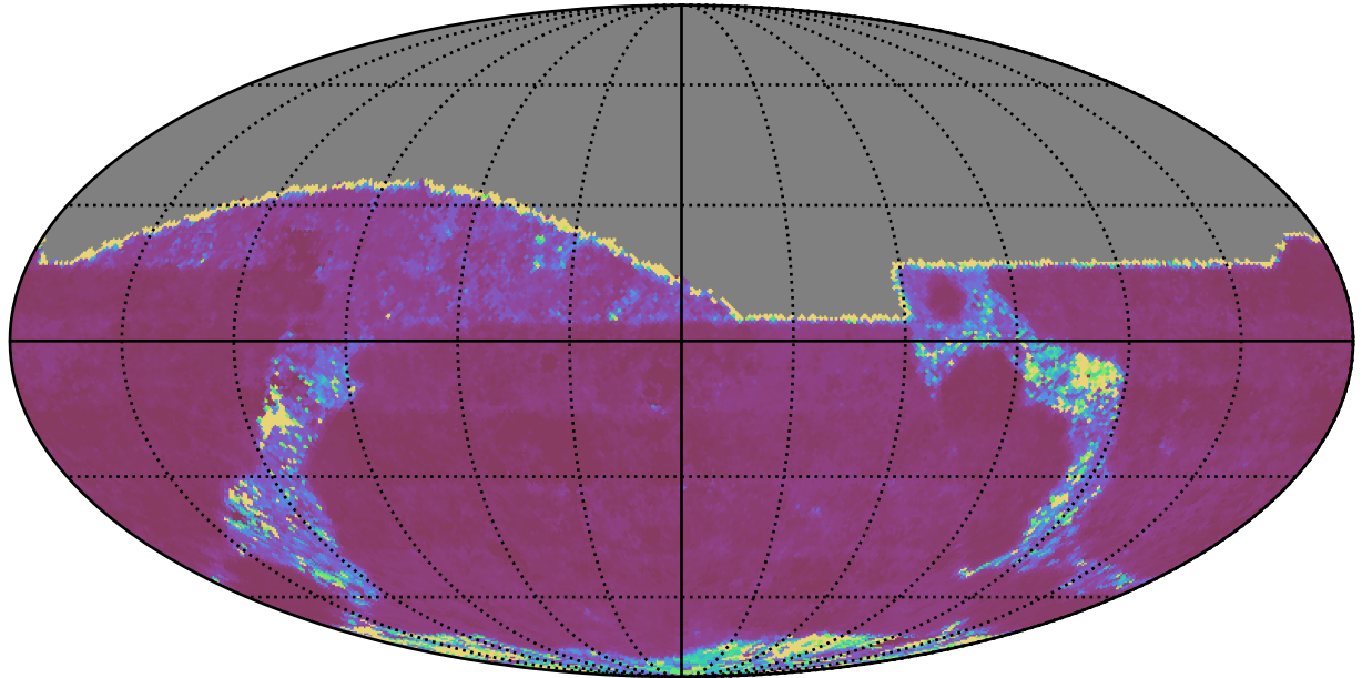
too_elab_heavy_r32_d3_ugrizy_v3.4_10yrs All sky g band: Median Inter-Night Gap
