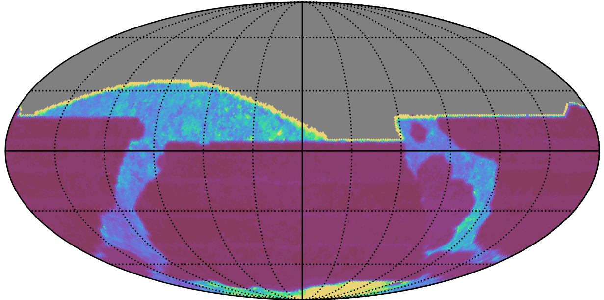
too_elab_heavy_r32_d3_ugrizy_v3.4_10yrs All sky all bands: Median Inter-Night Gap
