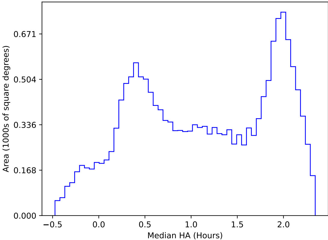
too_elab_heavy_r32_d3_ugrizy_v3.4_10yrs WFD z band: Median HA
