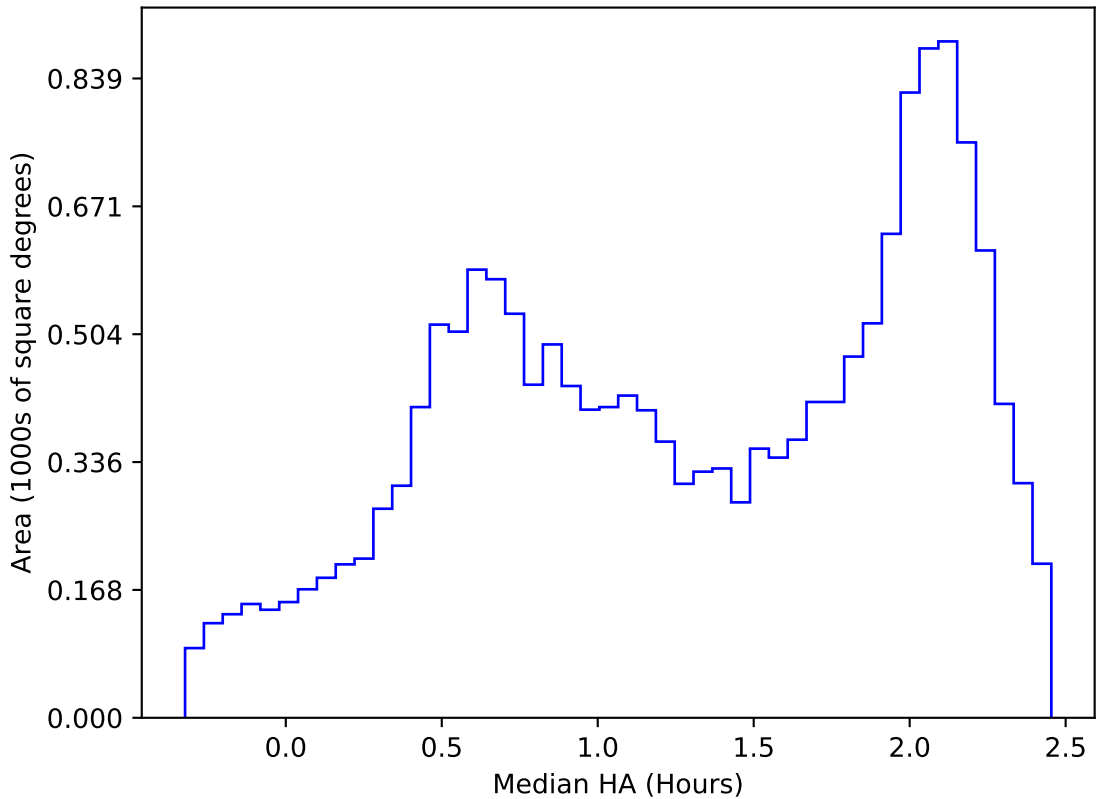
too_elab_heavy_r32_d3_ugrizy_v3.4_10yrs WFD y band: Median HA
