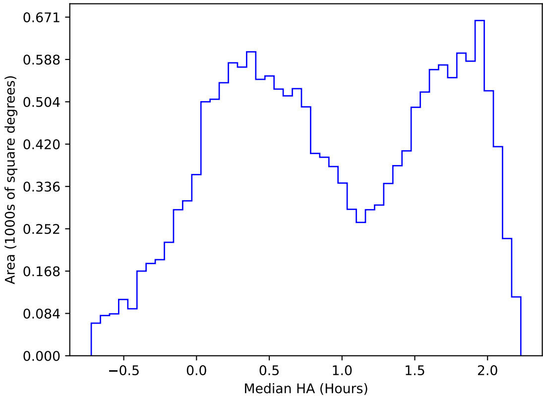
too_elab_heavy_r32_d3_ugrizy_v3.4_10yrs WFD r band: Median HA
