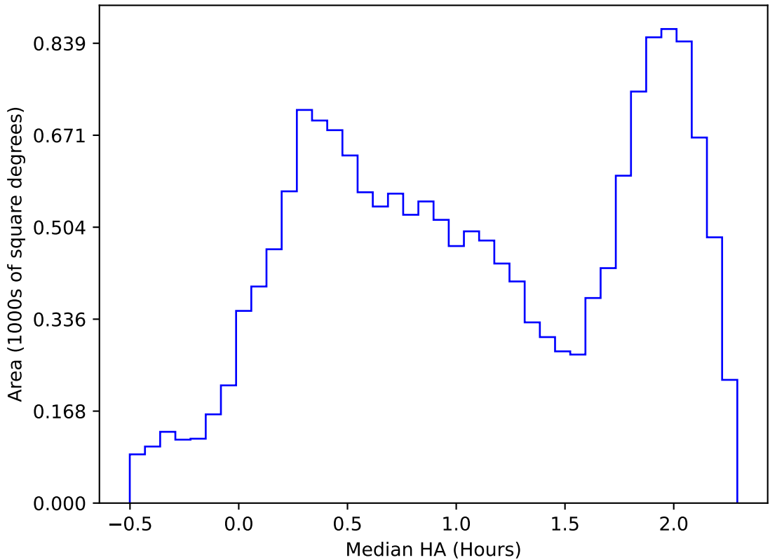
too_elab_heavy_r32_d3_ugrizy_v3.4_10yrs WFD i band: Median HA
