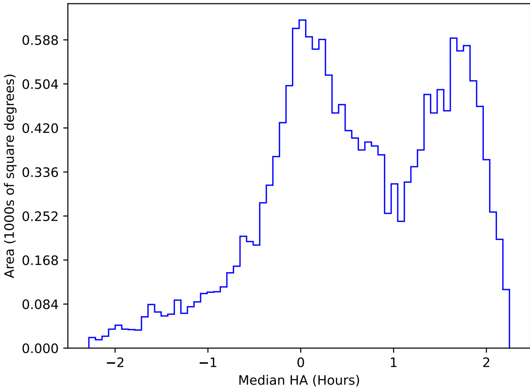
too_elab_heavy_r32_d3_ugrizy_v3.4_10yrs WFD g band: Median HA
