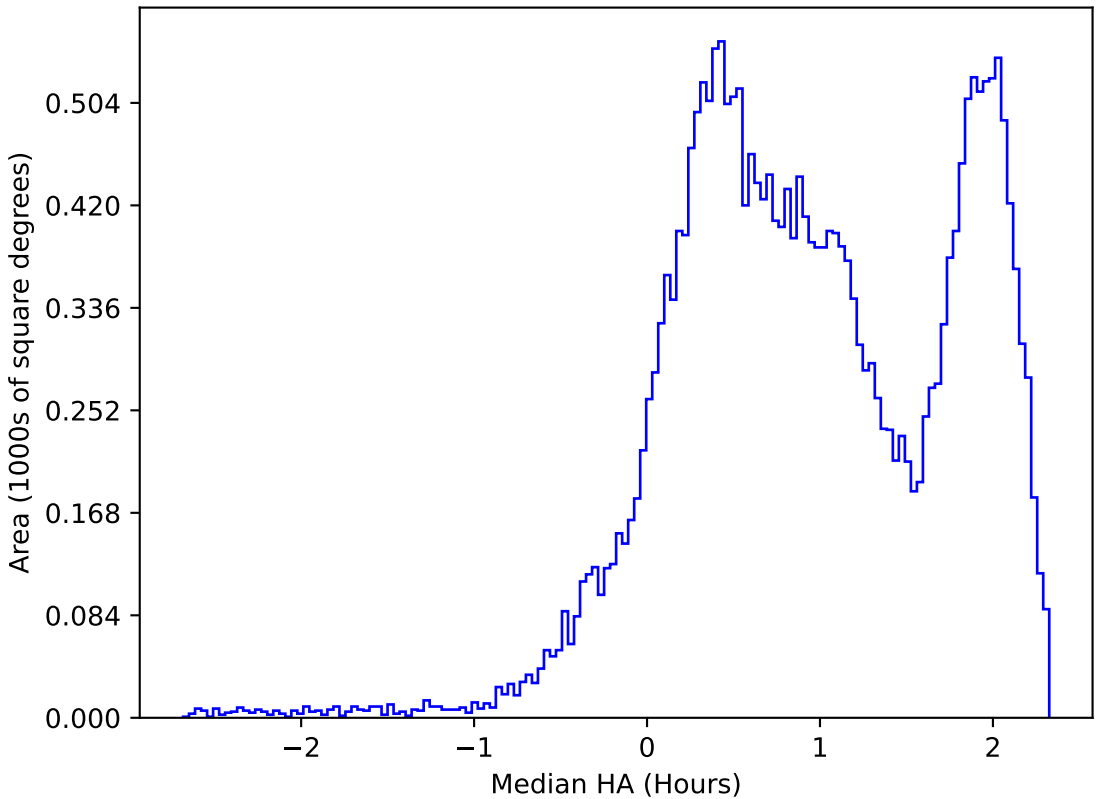
too_elab_heavy_r32_d3_ugrizy_v3.4_10yrs All sky i band: Median HA
