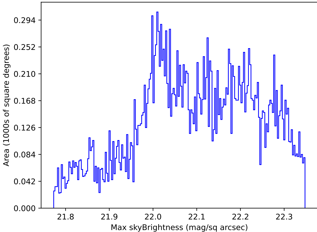
too_elab_heavy_r32_d3_ugrizy_v3.4_10yrs Yr 1 g band: Max skyBrightness
