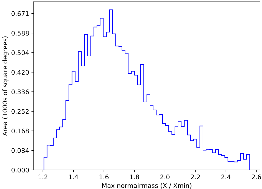
too_elab_heavy_r32_d3_ugrizy_v3.4_10yrs WFD u band: Max normairmass
