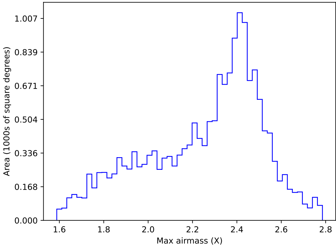
too_elab_heavy_r32_d3_ugrizy_v3.4_10yrs WFD r band: Max airmass
