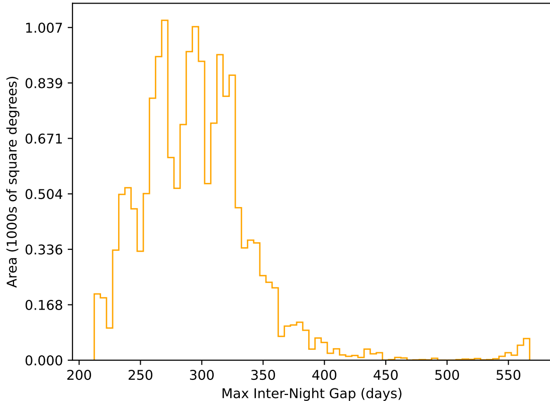
too_elab_heavy_r32_d3_ugrizy_v3.4_10yrs WFD r band: Max Inter-Night Gap
