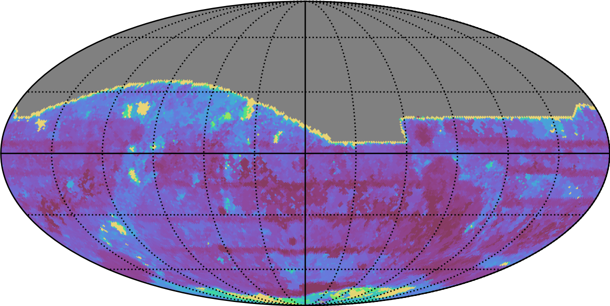
too_elab_heavy_r32_d3_ugrizy_v3.4_10yrs All sky all bands: Max Inter-Night Gap
