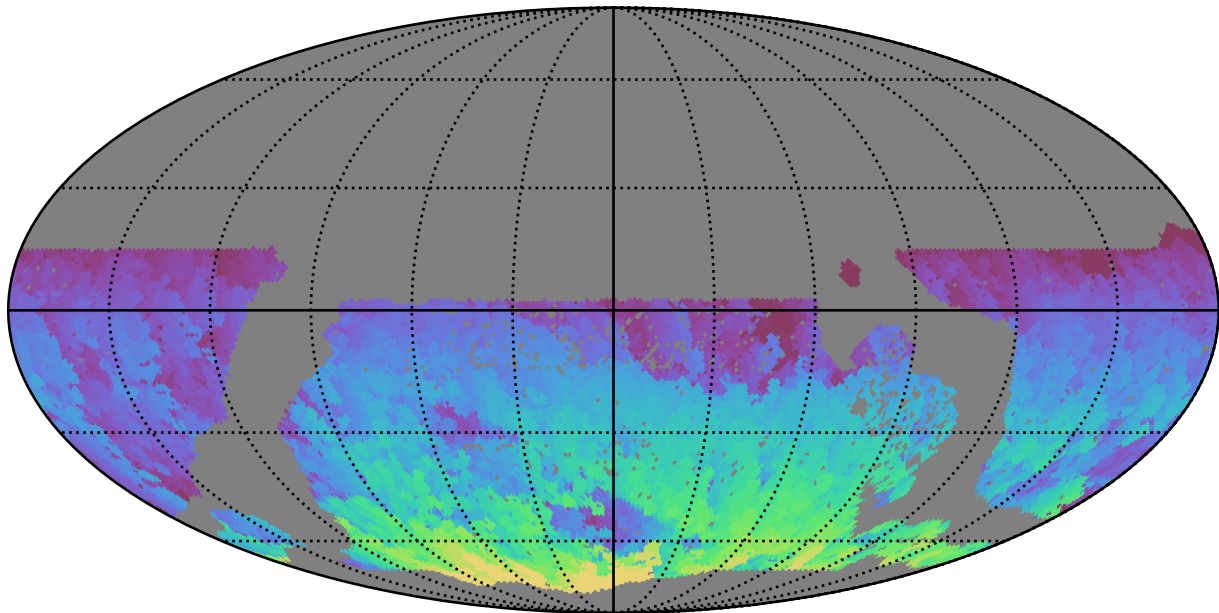
too_elab_heavy_r32_d3_ugrizy_v3.4_10yrs WFD z band: Max HA
