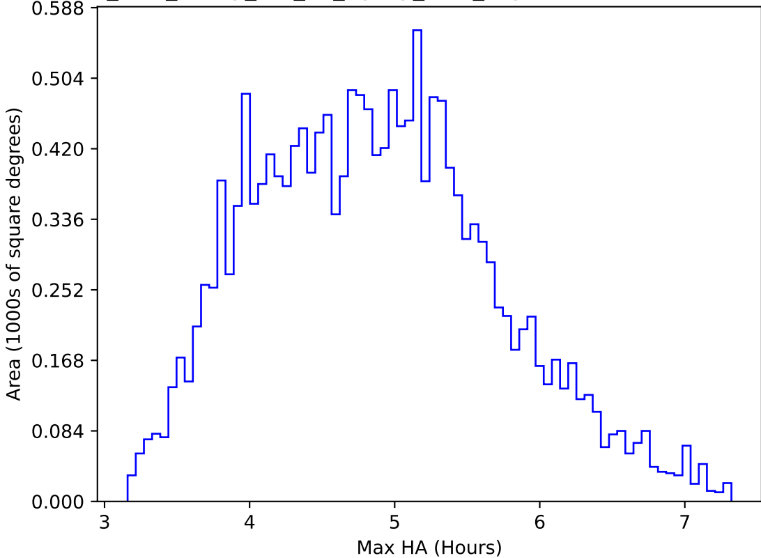
too_elab_heavy_r32_d3_ugrizy_v3.4_10yrs WFD z band: Max HA
