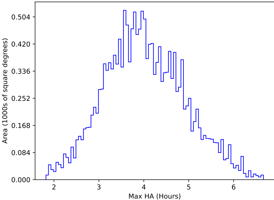
too_elab_heavy_r32_d3_ugrizy_v3.4_10yrs WFD u band: Max HA
