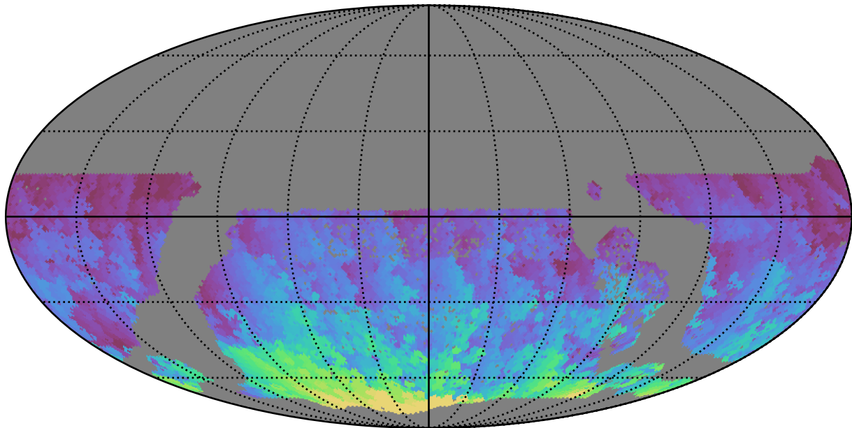
too_elab_heavy_r32_d3_ugrizy_v3.4_10yrs WFD r band: Max HA
