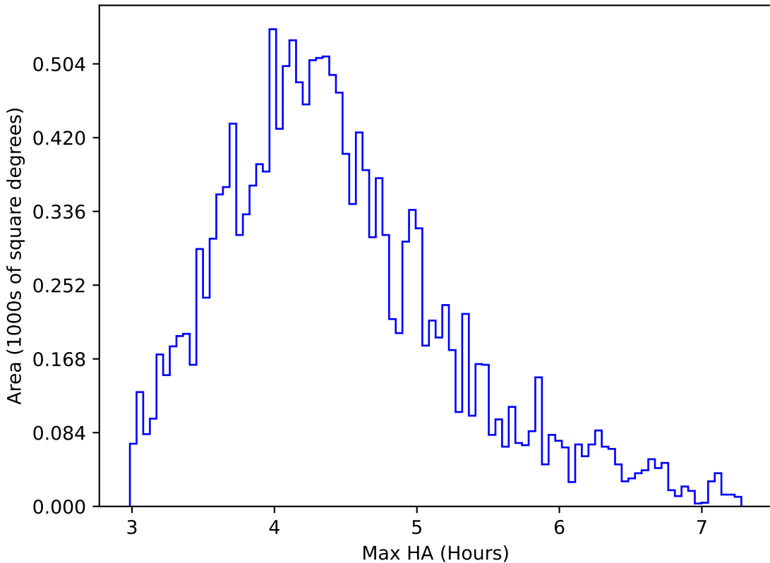
too_elab_heavy_r32_d3_ugrizy_v3.4_10yrs WFD r band: Max HA
