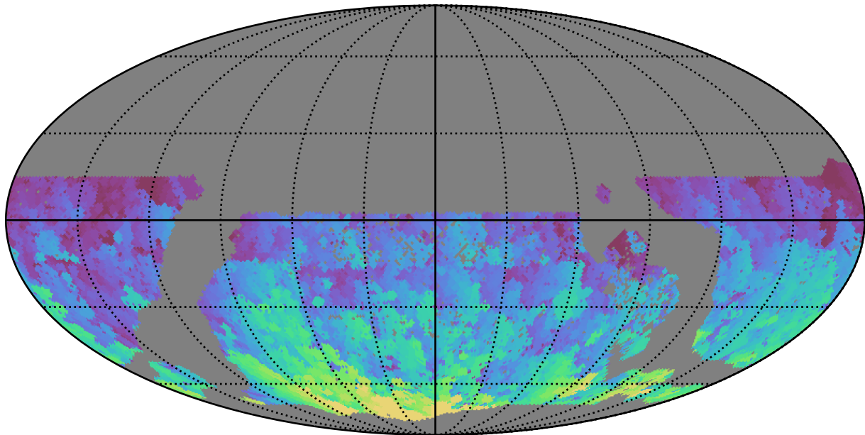
too_elab_heavy_r32_d3_ugrizy_v3.4_10yrs WFD g band: Max HA
