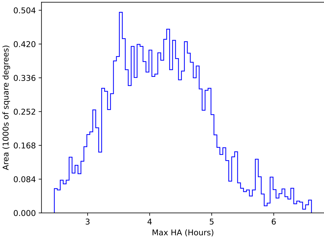
too_elab_heavy_r32_d3_ugrizy_v3.4_10yrs WFD g band: Max HA
