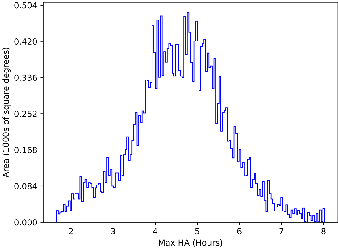
too_elab_heavy_r32_d3_ugrizy_v3.4_10yrs All sky z band: Max HA
