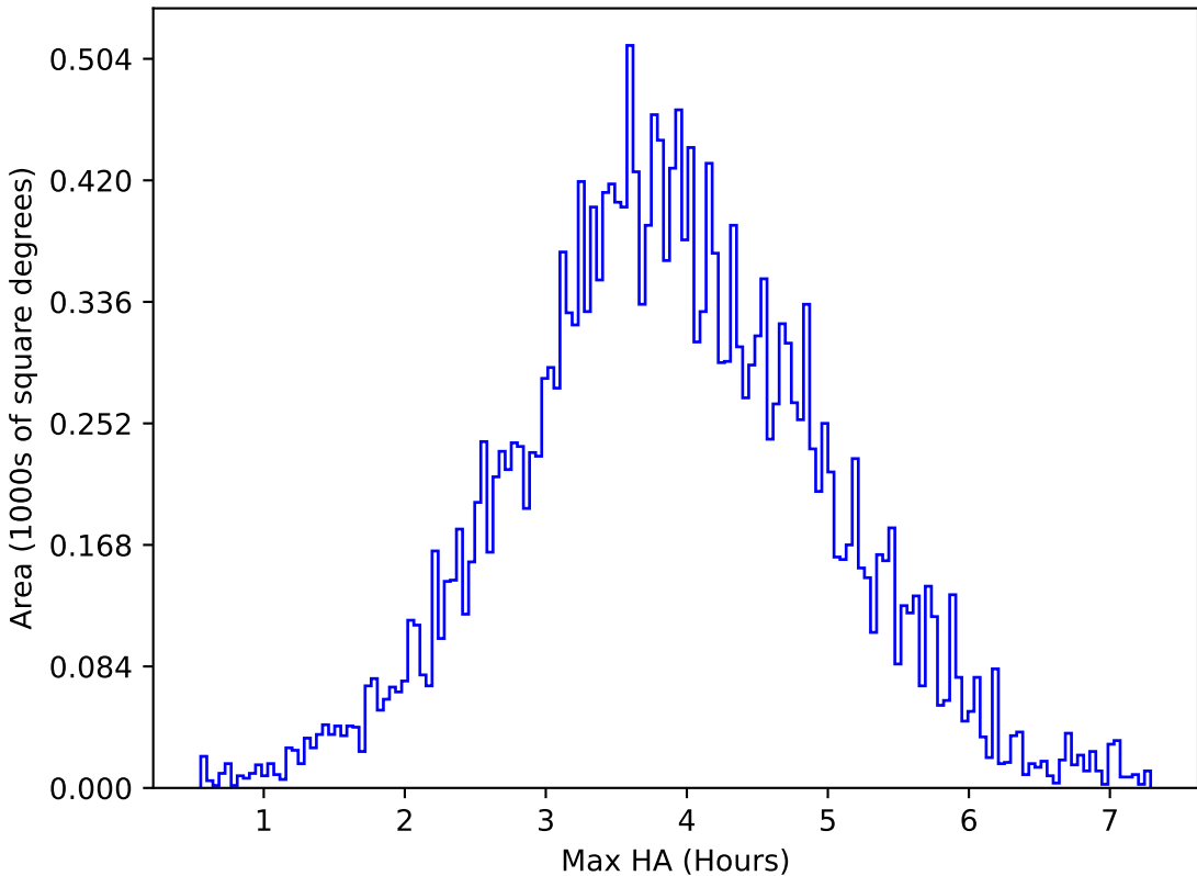
too_elab_heavy_r32_d3_ugrizy_v3.4_10yrs All sky u band: Max HA
