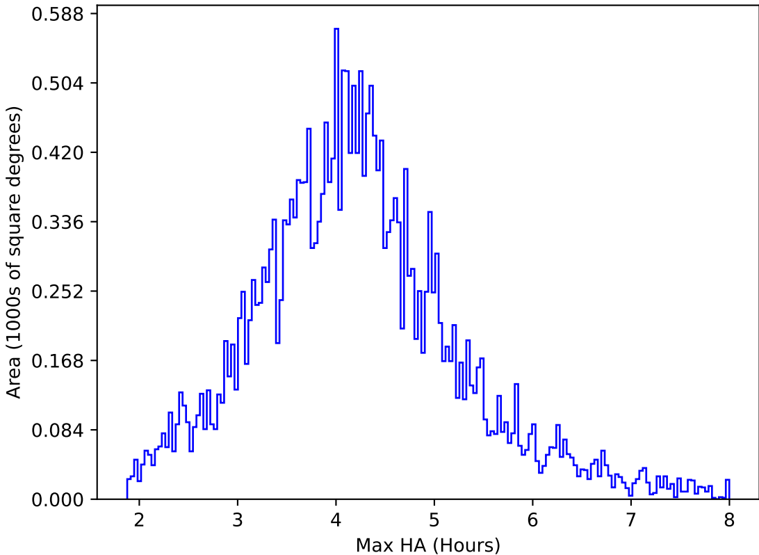
too_elab_heavy_r32_d3_ugrizy_v3.4_10yrs All sky r band: Max HA
