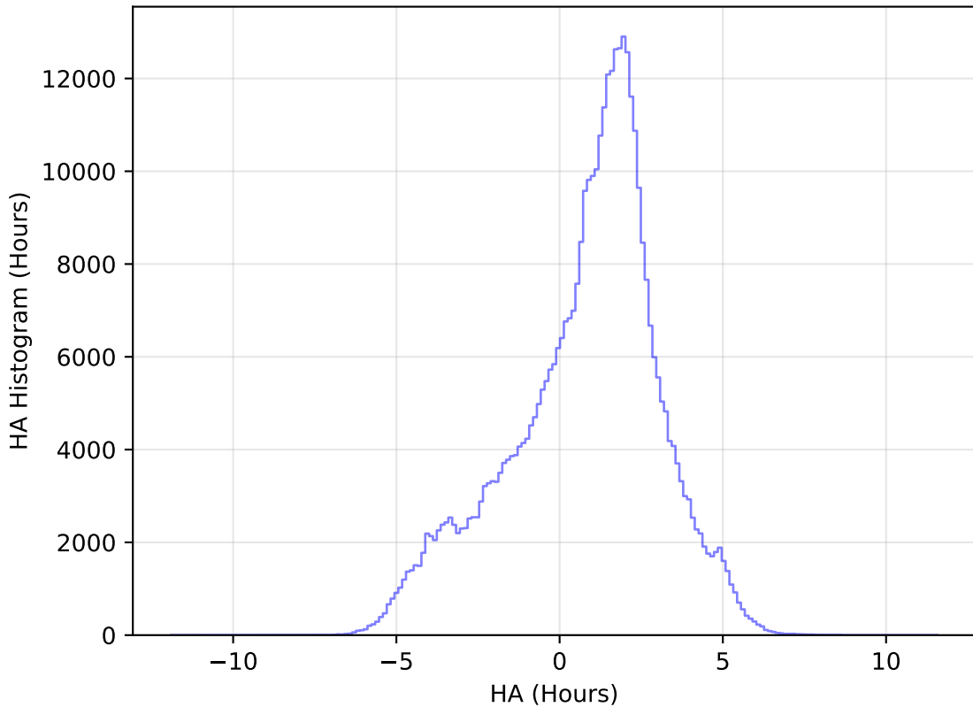
too_elab_heavy_r32_d3_ugrizy_v3.4_10yrs WFD z band: HA Histogram
