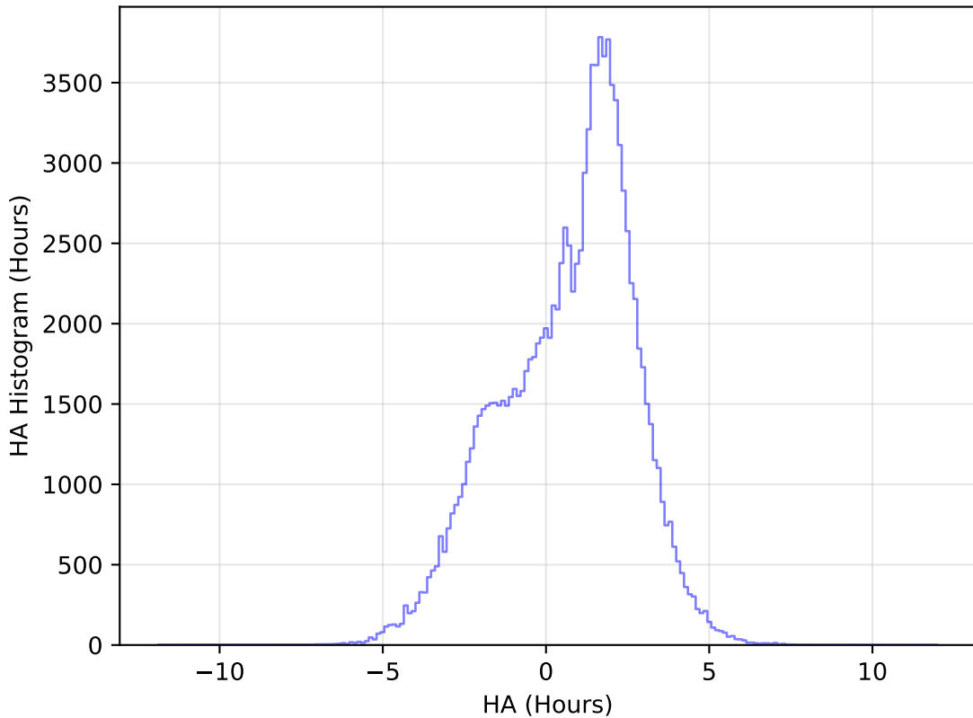
too_elab_heavy_r32_d3_ugrizy_v3.4_10yrs WFD u band: HA Histogram
