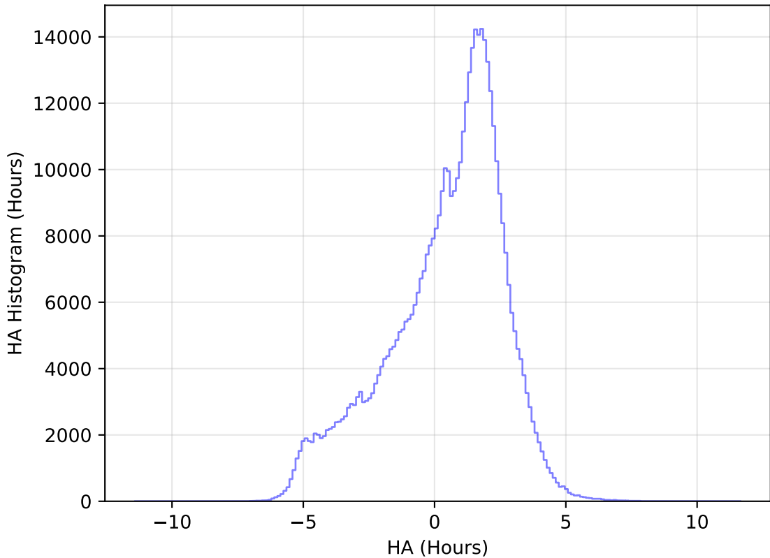
too_elab_heavy_r32_d3_ugrizy_v3.4_10yrs WFD r band: HA Histogram
