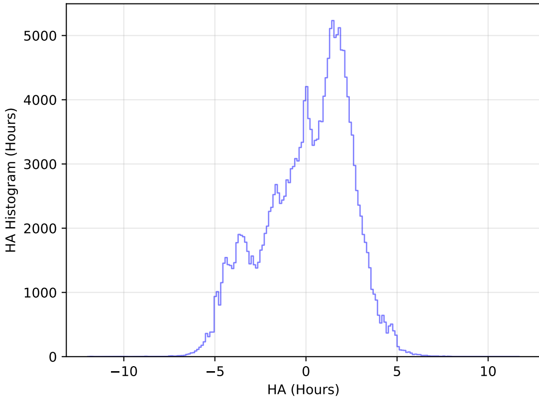
too_elab_heavy_r32_d3_ugrizy_v3.4_10yrs WFD g band: HA Histogram
