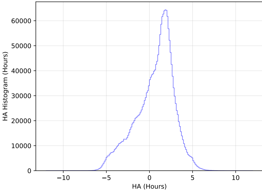
too_elab_heavy_r32_d3_ugrizy_v3.4_10yrs WFD all bands: HA Histogram
