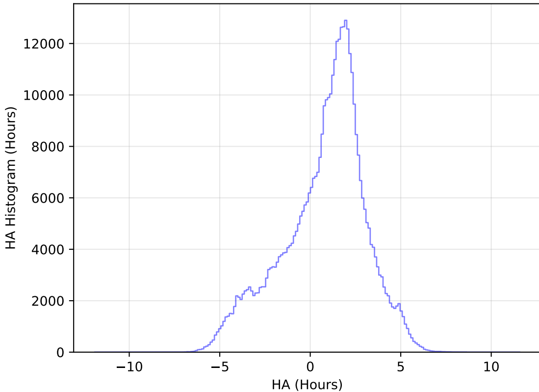
too_elab_heavy_r32_d3_ugrizy_v3.4_10yrs All sky z band: HA Histogram
