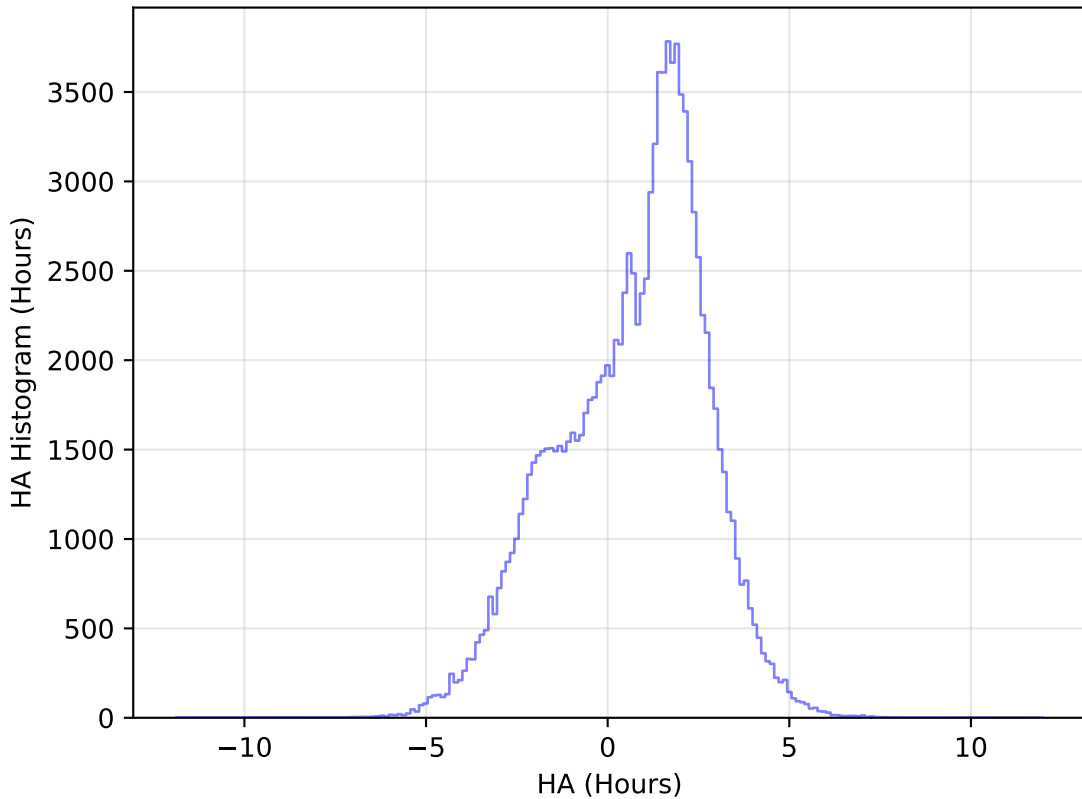
too_elab_heavy_r32_d3_ugrizy_v3.4_10yrs All sky u band: HA Histogram
