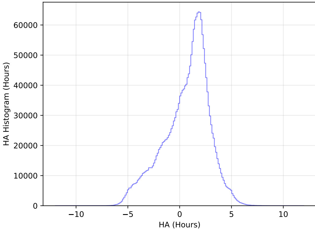
too_elab_heavy_r32_d3_ugrizy_v3.4_10yrs All sky all bands: HA Histogram
