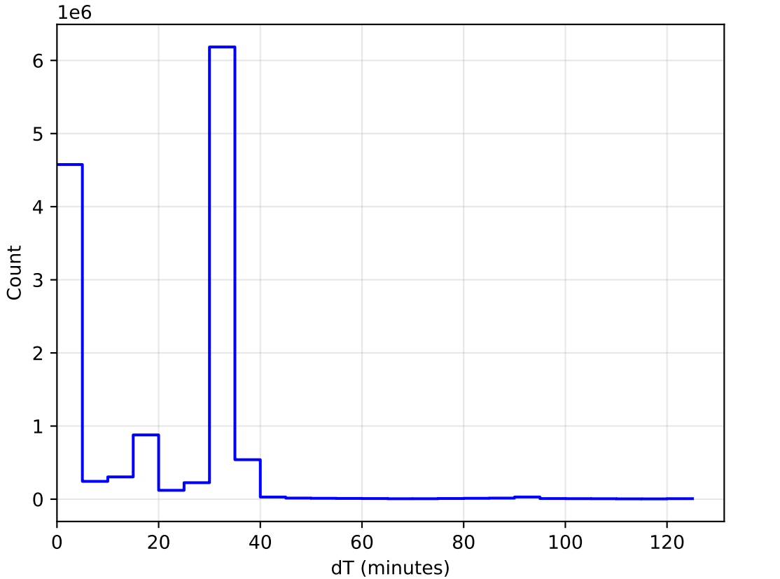
too_elab_heavy_r32_d3_ugrizy_v3.4_10yrs All sky: DeltaT Histogram
