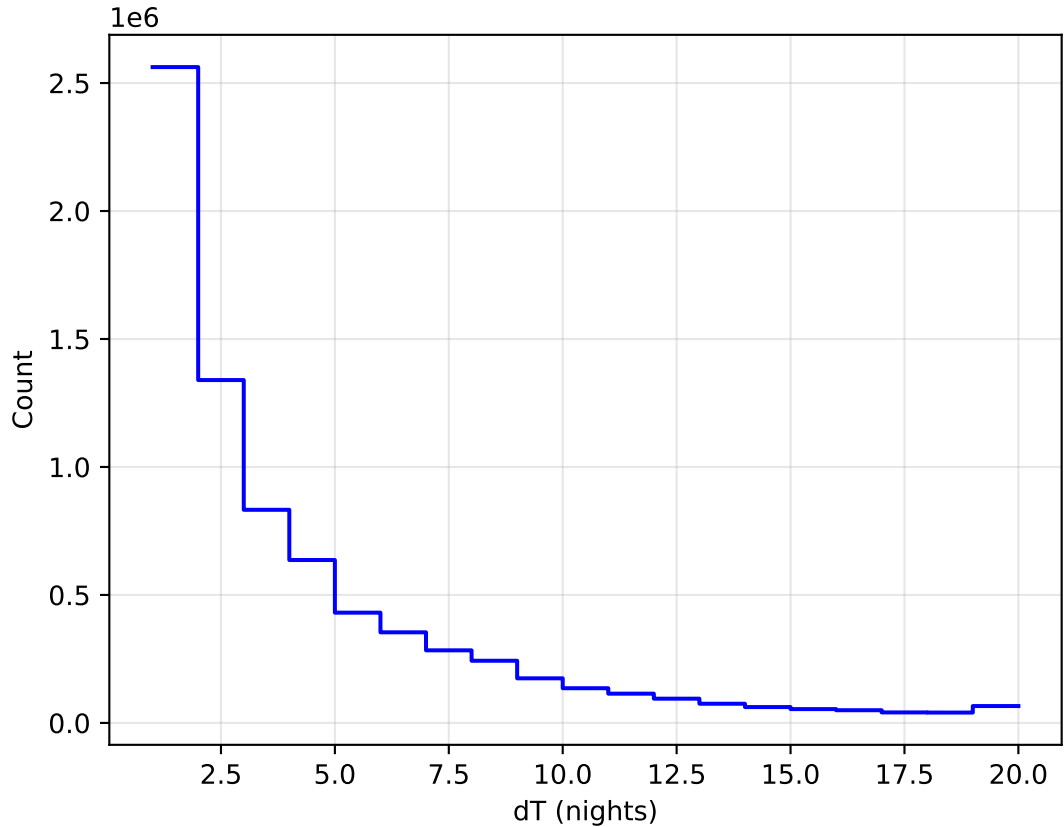
too_elab_heavy_r32_d3_ugrizy_v3.4_10yrs WFD all bands: DeltaNight Histogram
