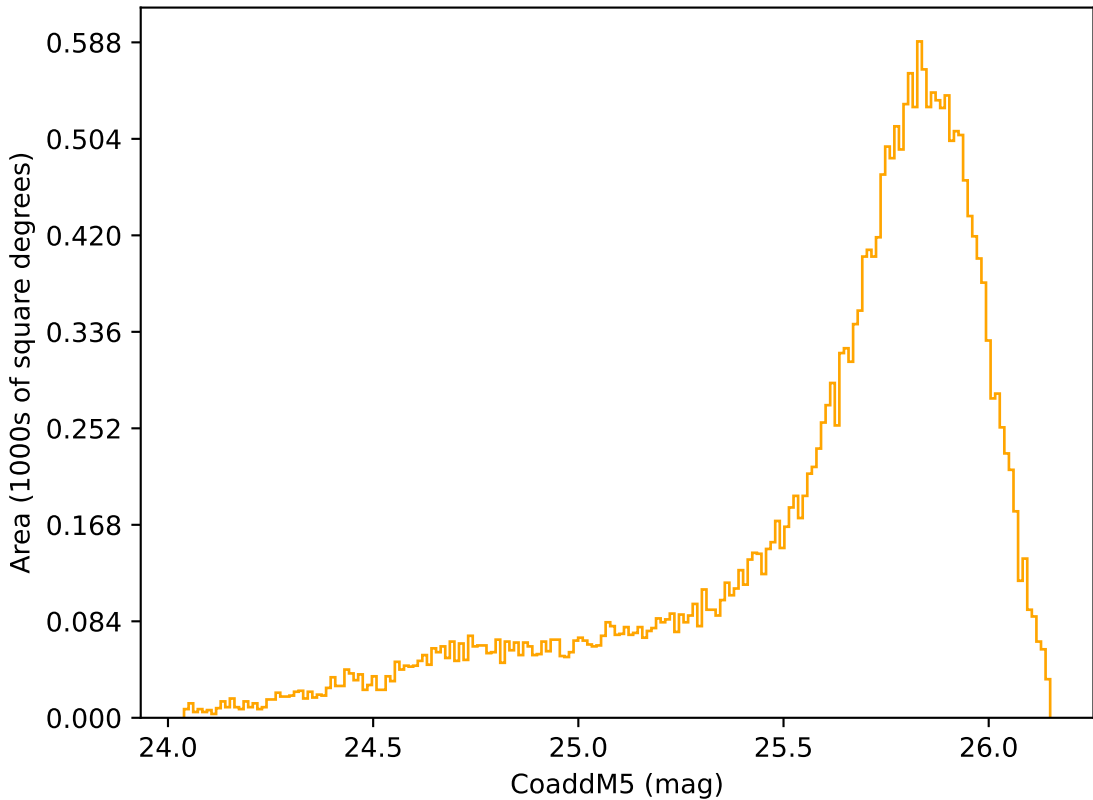
too_elab_heavy_r32_d3_ugrizy_v3.4_10yrs Yr 1 r band: CoaddM5
