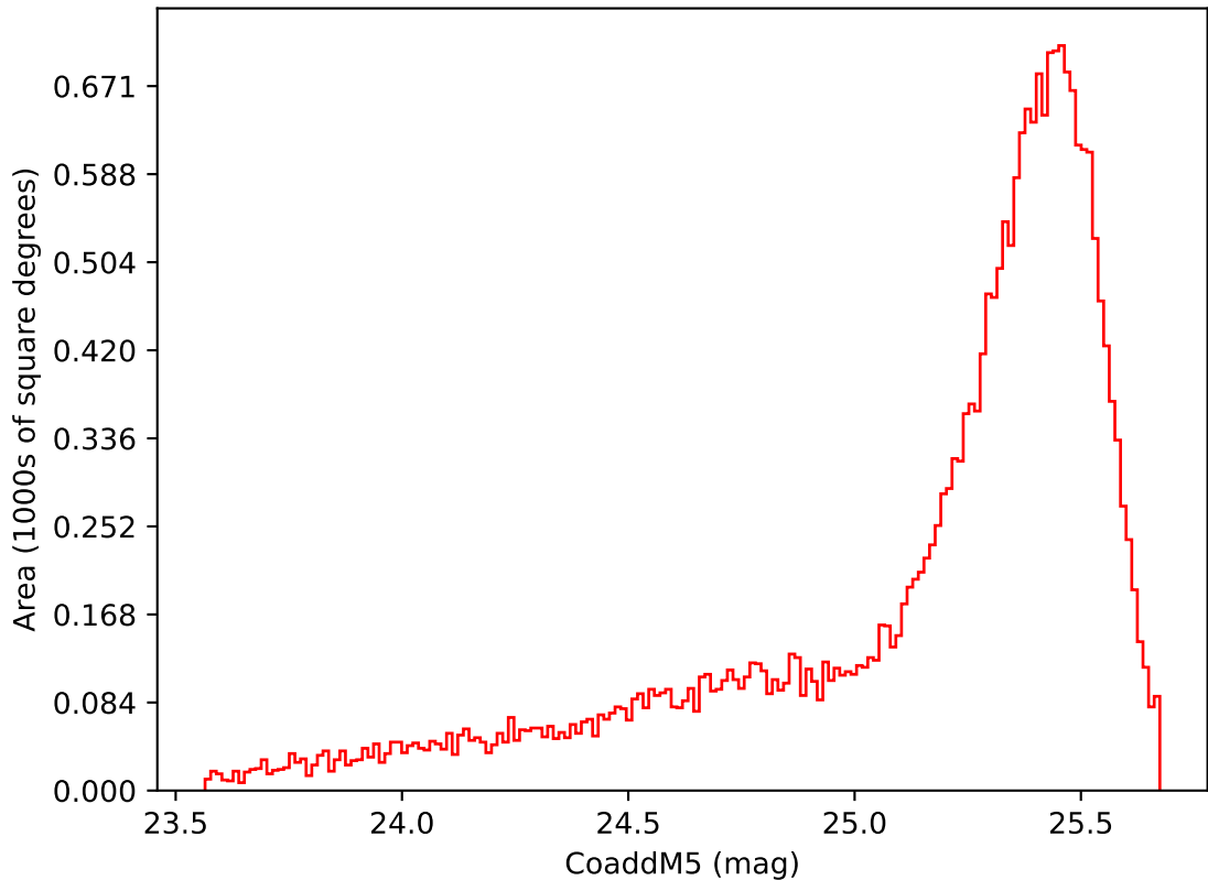
too_elab_heavy_r32_d3_ugrizy_v3.4_10yrs Yr 1 i band: CoaddM5
