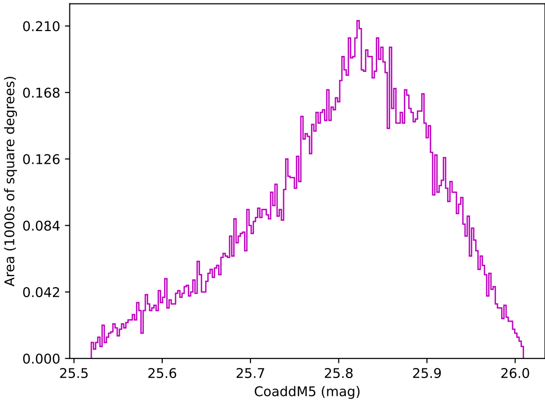
too_elab_heavy_r32_d3_ugrizy_v3.4_10yrs WFD z band: CoaddM5
