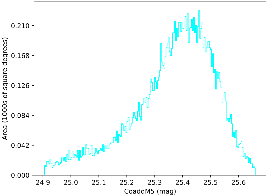
too_elab_heavy_r32_d3_ugrizy_v3.4_10yrs WFD u band: CoaddM5
