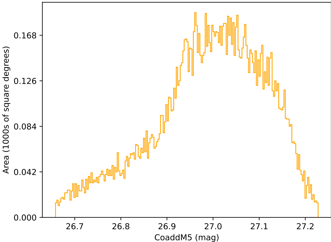
too_elab_heavy_r32_d3_ugrizy_v3.4_10yrs WFD r band: CoaddM5
