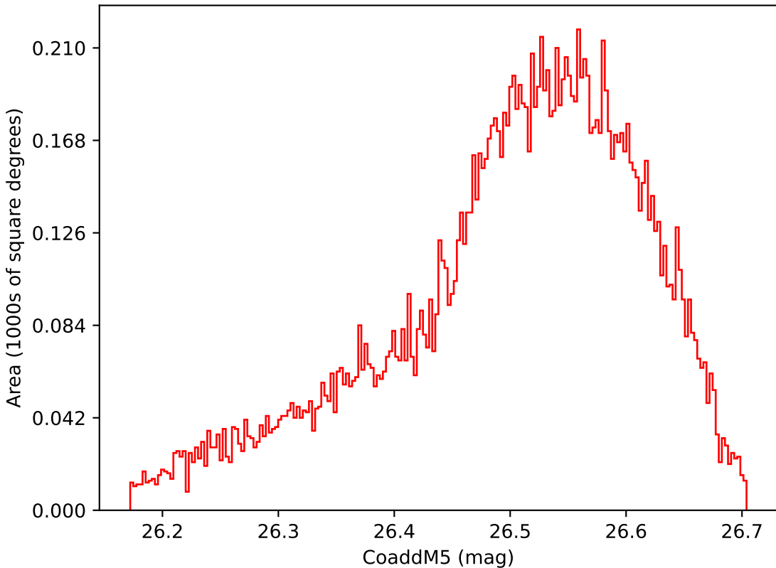
too_elab_heavy_r32_d3_ugrizy_v3.4_10yrs WFD i band: CoaddM5
