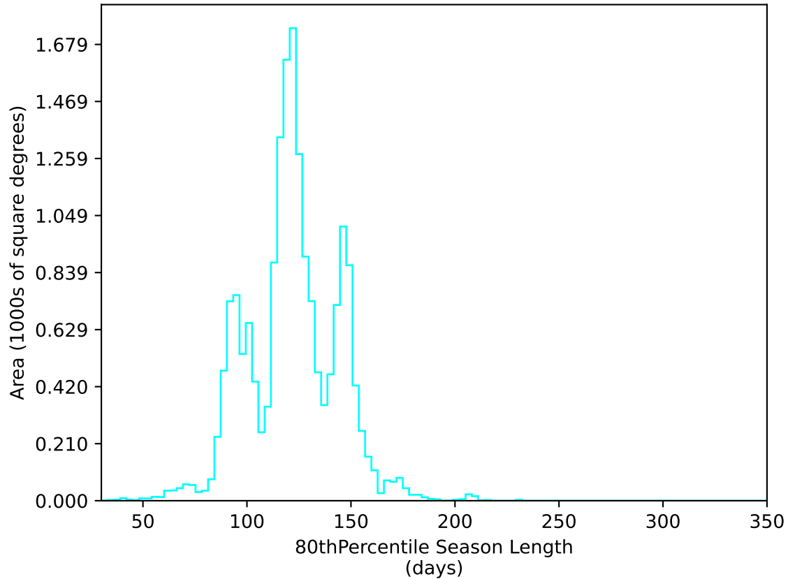
too_elab_heavy_r32_d3_ugrizy_v3.4_10yrs WFD u band: 80thPercentile Season Length
