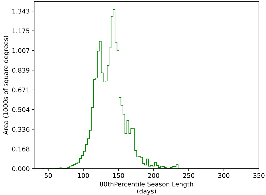
too_elab_heavy_r32_d3_ugrizy_v3.4_10yrs WFD g band: 80thPercentile Season Length
