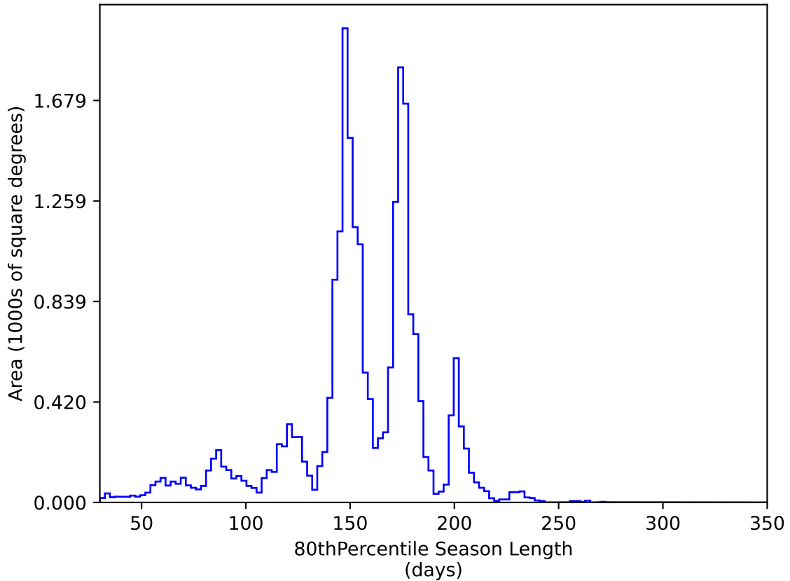
too_elab_heavy_r32_d3_ugrizy_v3.4_10yrs All sky y band: 80thPercentile Season Length
